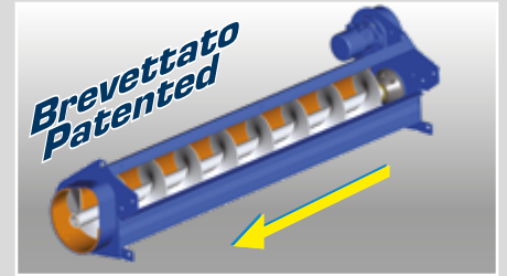
Coclee coassiali con spirali opposte per la pacciamatura da ambo i lati. Coaxial spirals with opposite helixes for mulched stubble delivery on both sides.
